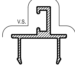
ME7 45mm DOOR STOP Mass. 0.275 Kg/m Anod. Per. 138 Paint Per. 100
