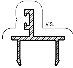
ME40 40mm DOOR STOP Mass. 0.271 Kg/m Anod. Per. 136 Paint Per. 100
