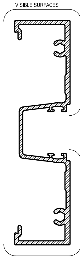
ME24 25mm NARROW FRAME Mass. 1.140 Kg/m Anod. Per. 468 Paint Per. 127
