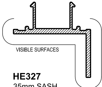
HE327 35mm SASH ADAPTOR Mass. 0.395 Kg/m Anod. Per. 171 Paint Per. 100
