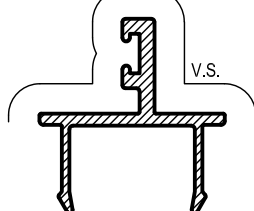
ME45 45mm DOOR STOP Mass. 0.271 Kg/m Anod. Per. 136 Paint Per. 100
