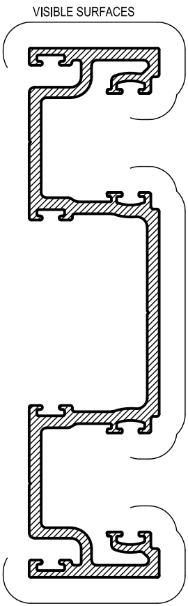
HE903 ACOUSTIC FEMALE MULLION Mass. 1.482 Kg/m Anod. Per. 544 Paint Per. 125 Ixx = 665.42 x 10 3 mm 4
