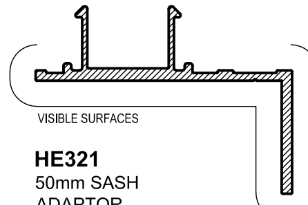
HE321 50mm SASH ADAPTOR Mass. 0.470 Kg/m Anod. Per. 205 Paint Per. 100
