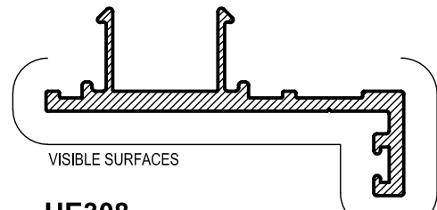
HE308 45mm DOOR STOP Mass. 0.579 Kg/m Anod. Per. 212 Paint Per. 100
